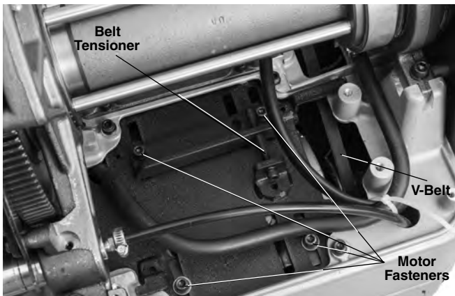
Figure 35 – Belt Tensioning
