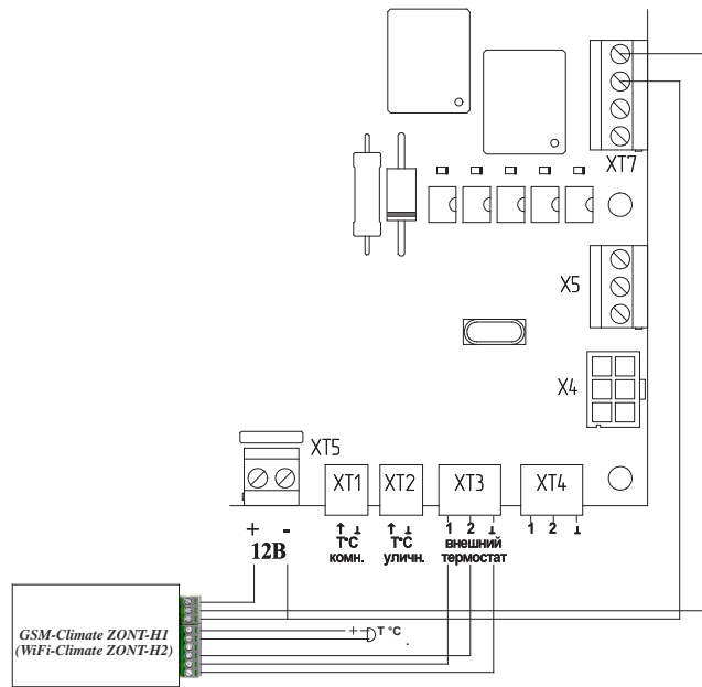
23 GSM-Climate, WiFi-Climate "ZONT EXPERT"
