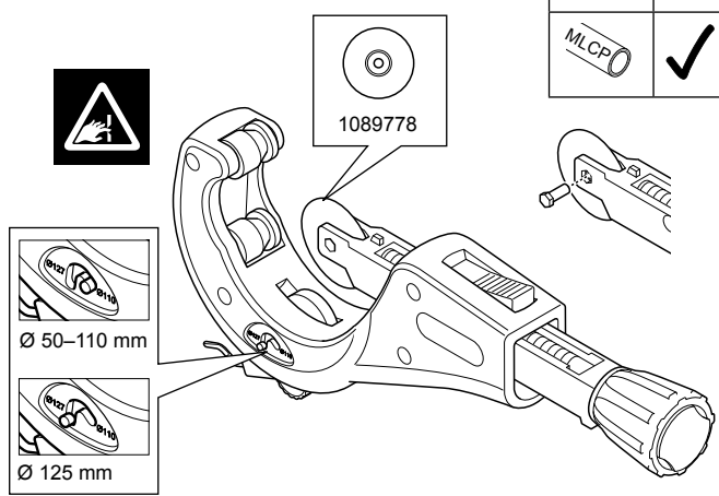
Uponor Multi pipe cutting tool 50–125 mm (1089676)
