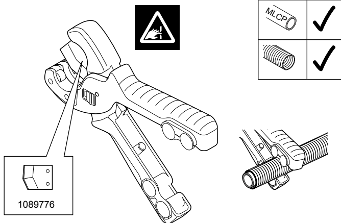
Uponor Multi pipe & conduit cutting tool 12–25 mm (1089674)
