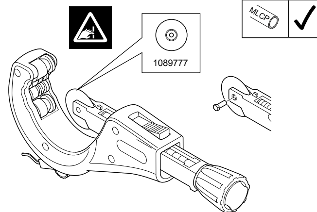
Uponor Multi pipe cutting tool 25–63 mm (1089675)
