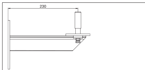
Dimensions wall bracket for 2- and 3-fold distributors
