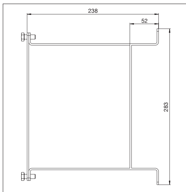
Dimensions wall bracket
