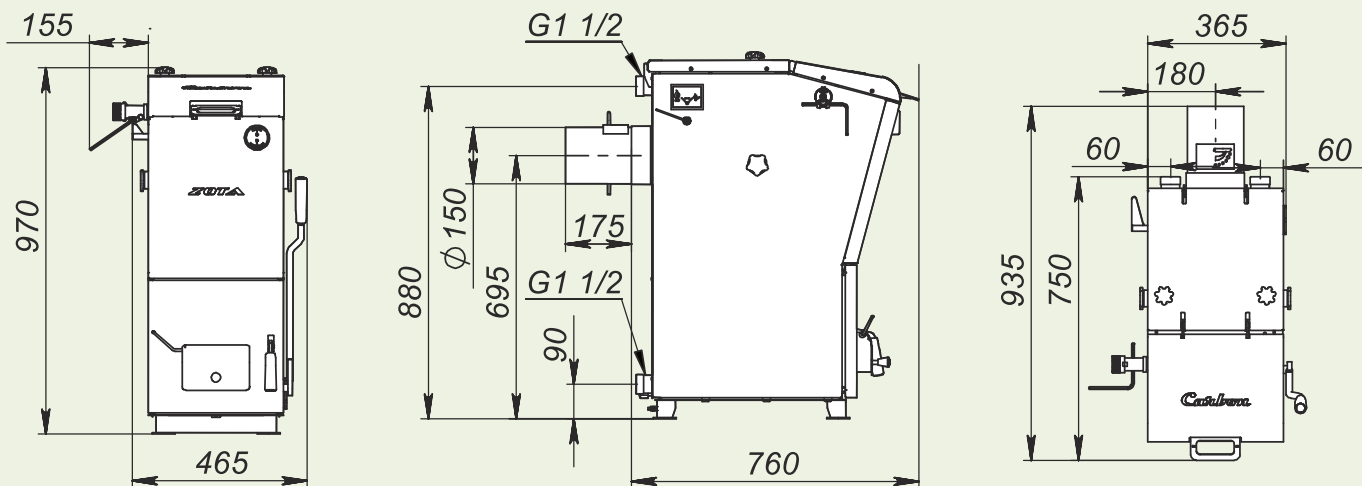
ZOTA "Carbon"-15
