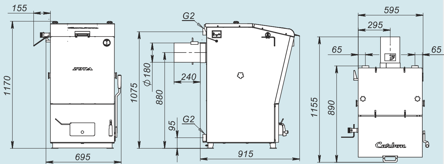
ZOTA "Carbon"-50
