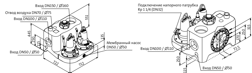
MULTILIFT MDG
