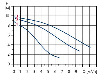
UPS 32-100 180
