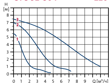
UPS 32-80 F 220
