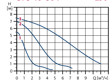
UPS 40-80 F 250
