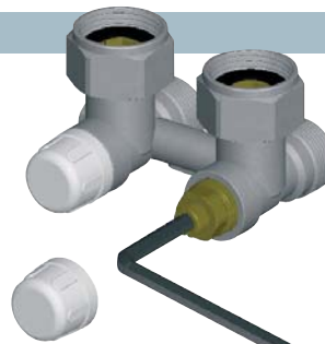
LOCKSHIELD VALVE REGULATION
