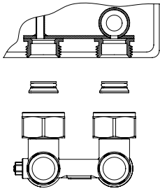
SECTIONED RADIATOR
